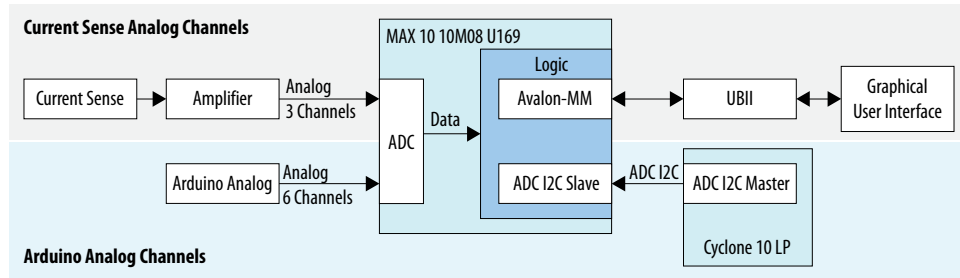
Figure 13. Current Measurement
