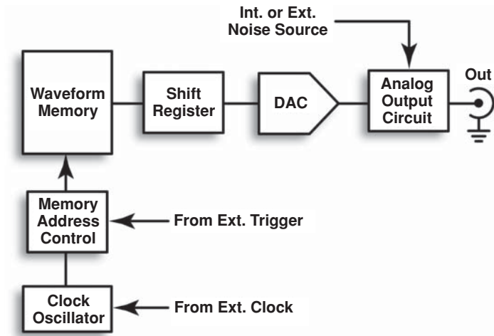
Figure 18. The architecture of an arbitrary waveform generator (simplified).
